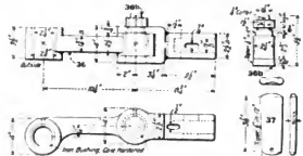
Figs. 2089-2094. Valve Rod for Ten-Wheel (1-4-0) Locomotive. Lehigh Valley.
